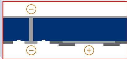
Cross-Section: Metal Wrap Through (MWT).
